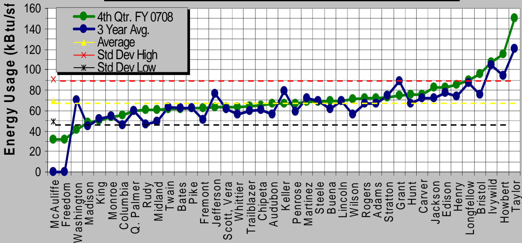
D-11 Elementary Schools: 4th Quarter FY 07-08 Energy Use Index
