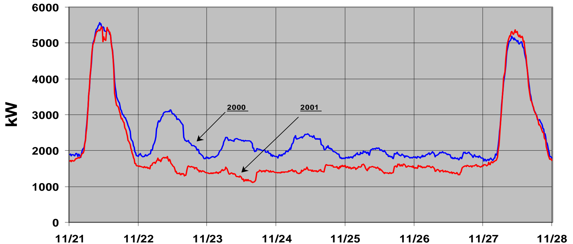
Thanksgiving Break Shutdown Electric Load Comparison Graph - All Sites
